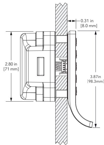
Side View-Cable
