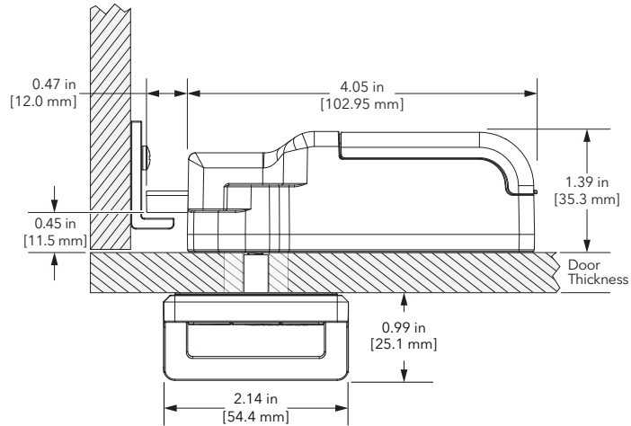
Top View-Cable
