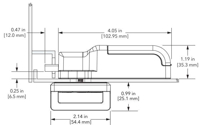
Top View-Pin Connector
